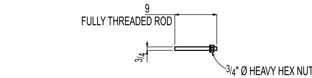
4 THREADED RODS F-08.02M5
